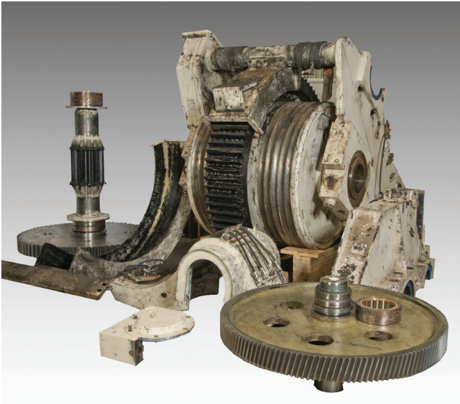
Electric Shovel Crowd Transmission (before)
